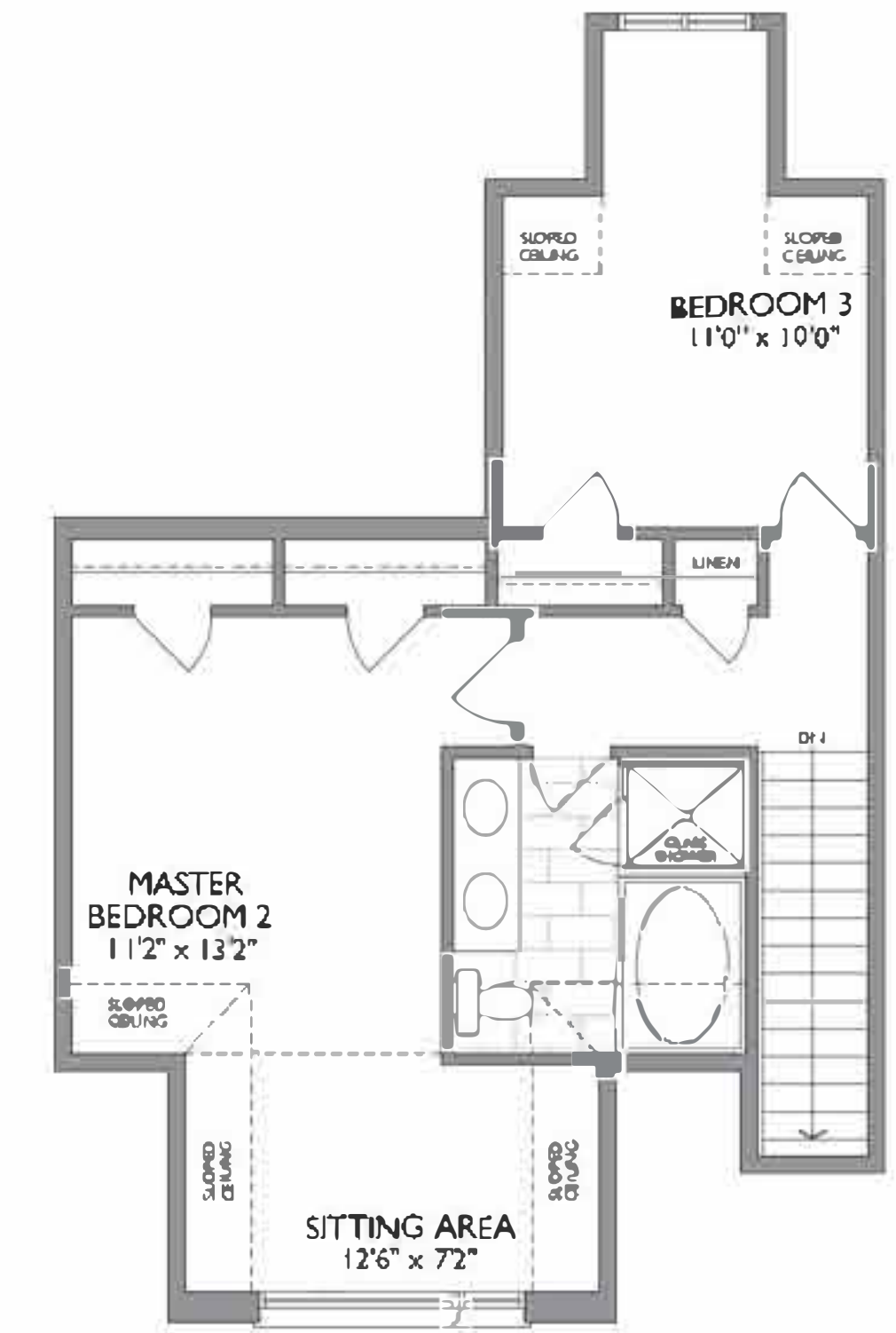
OPT. LOFT WITH MASTER BEDROOM 2 & BEDROOM 3
