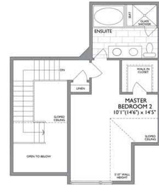
OPT. LOFT WITH MASTER BEDROOM 2 & END CONDITION
