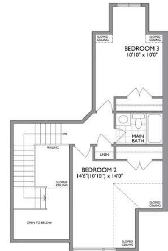
END CONDITION LOFT WITH BEDROOMS 3 & 4
